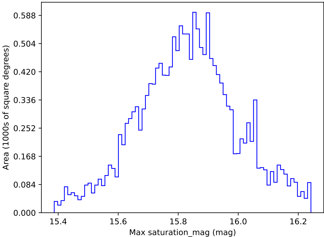
extra_ss_neo4_v3.4_10yrs WFD all bands: Max saturation_mag
