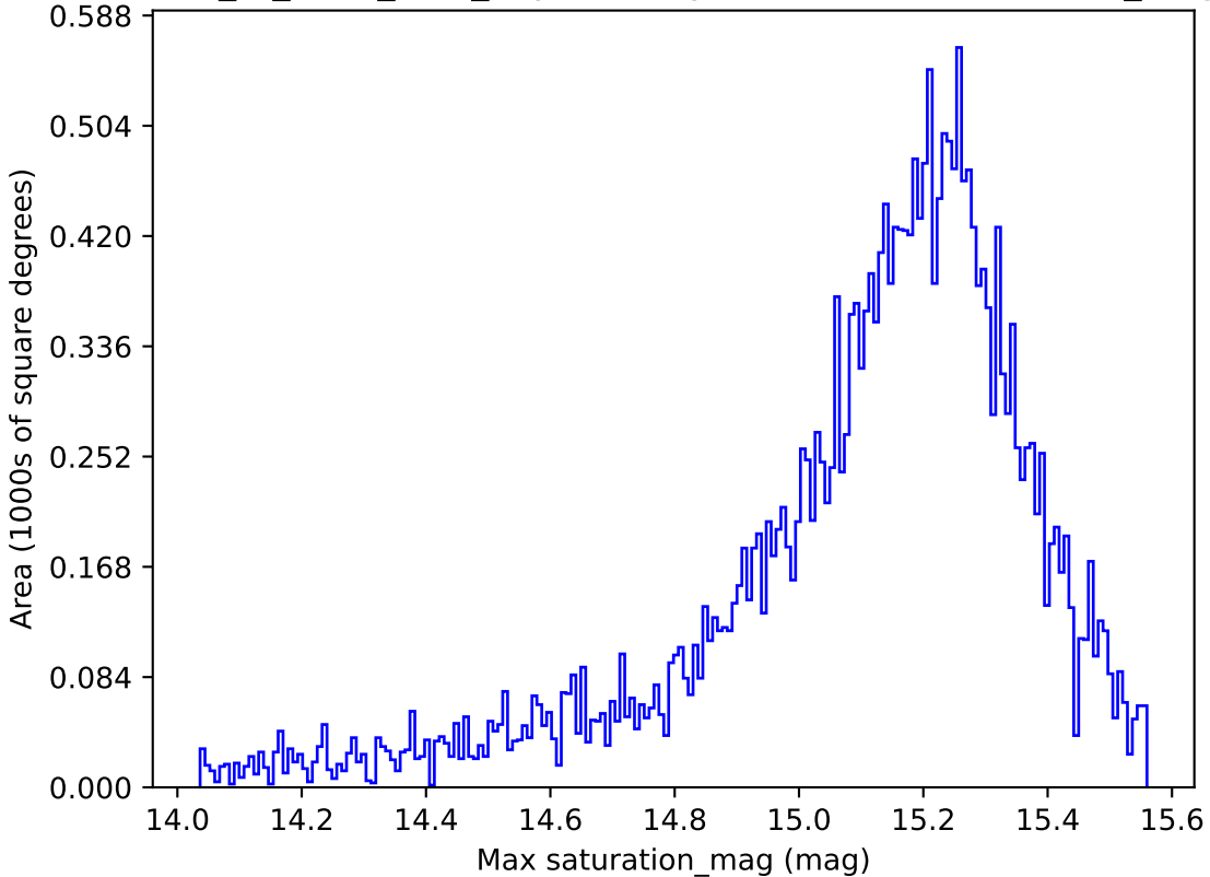
extra_ss_neo4_v3.4_10yrs All sky z band: Max saturation_mag
