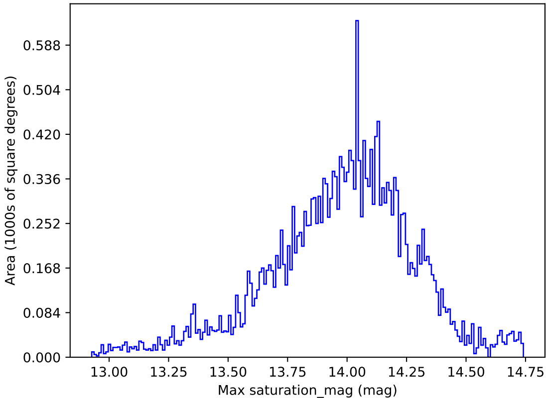
extra_ss_neo4_v3.4_10yrs All sky u band: Max saturation_mag
