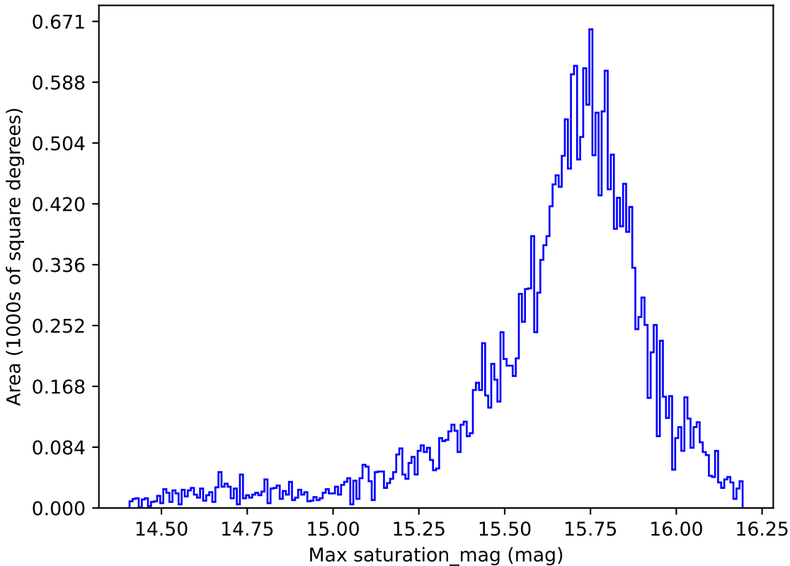
extra_ss_neo4_v3.4_10yrs All sky r band: Max saturation_mag
