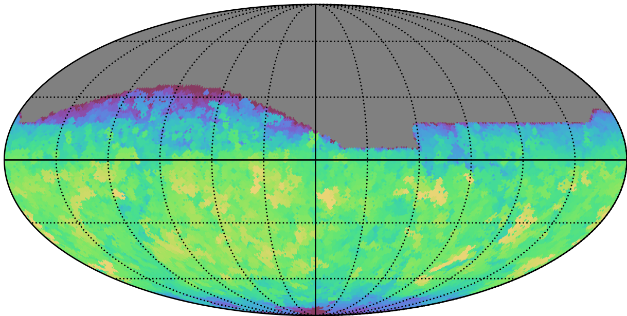
extra_ss_neo4_v3.4_10yrs All sky i band: Max saturation_mag
