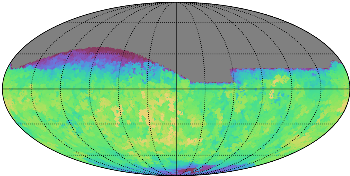
extra_ss_neo4_v3.4_10yrs All sky g band: Max saturation_mag
