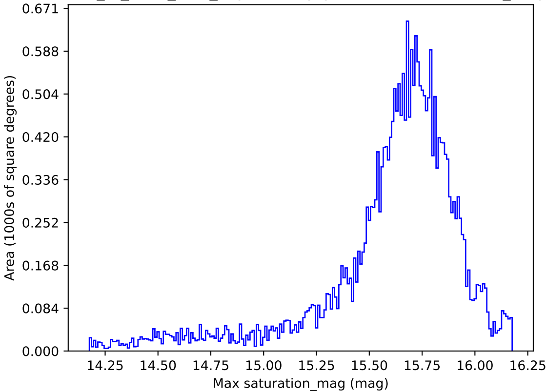
extra_ss_neo4_v3.4_10yrs All sky g band: Max saturation_mag
