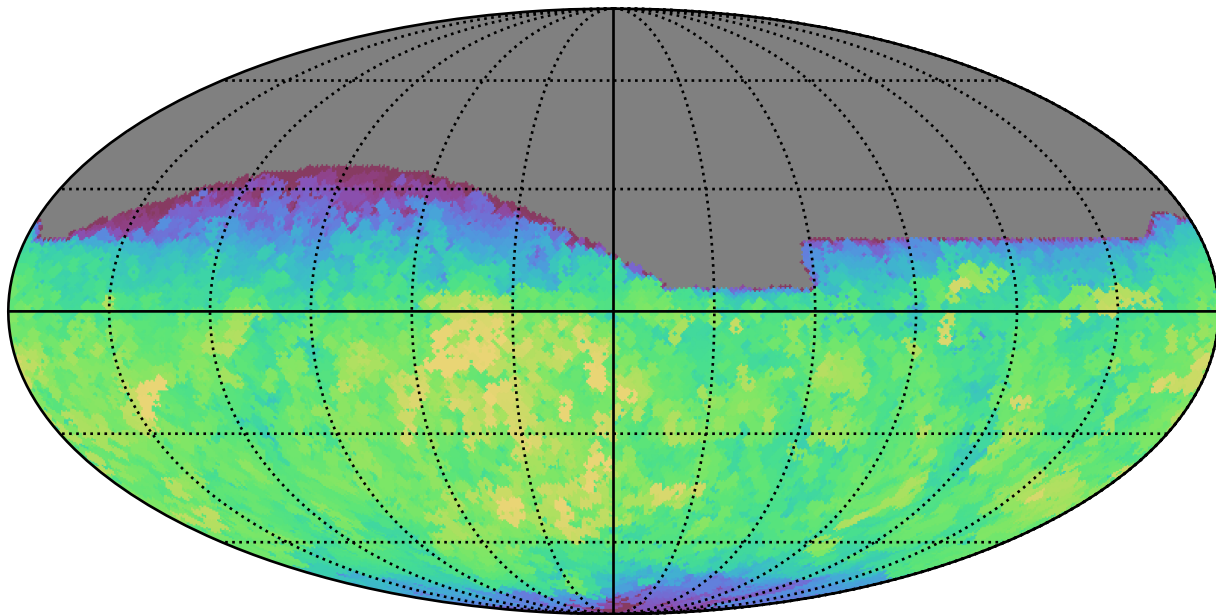
extra_ss_neo4_v3.4_10yrs All sky all bands: Max saturation_mag
