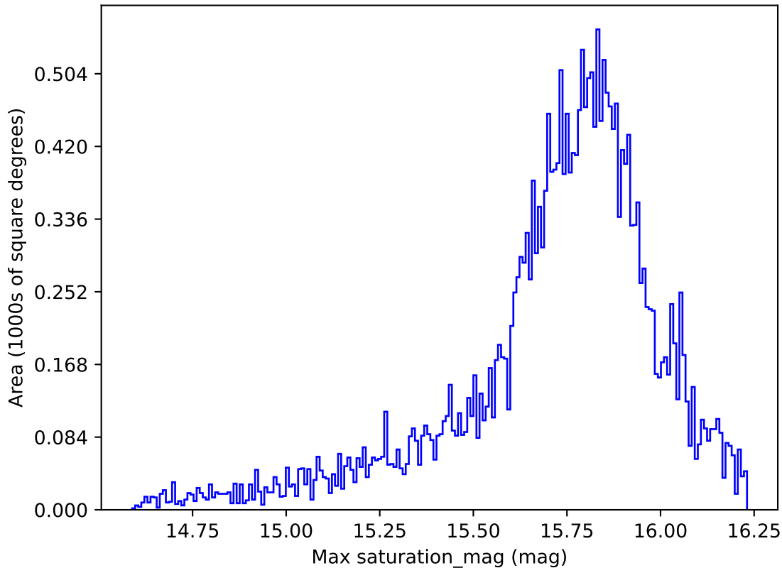
extra_ss_neo4_v3.4_10yrs All sky all bands: Max saturation_mag
