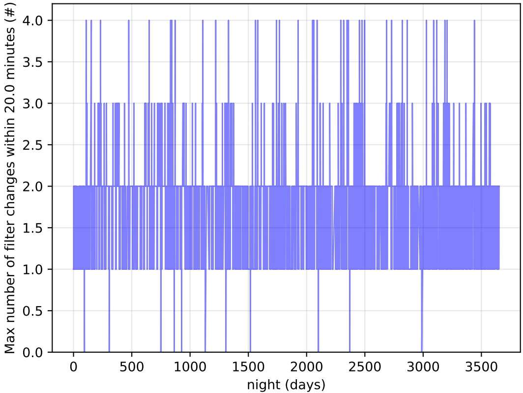
extra_ss_neo4_v3.4_10yrs Per Night: Max number of filter changes within 20.0 minutes
