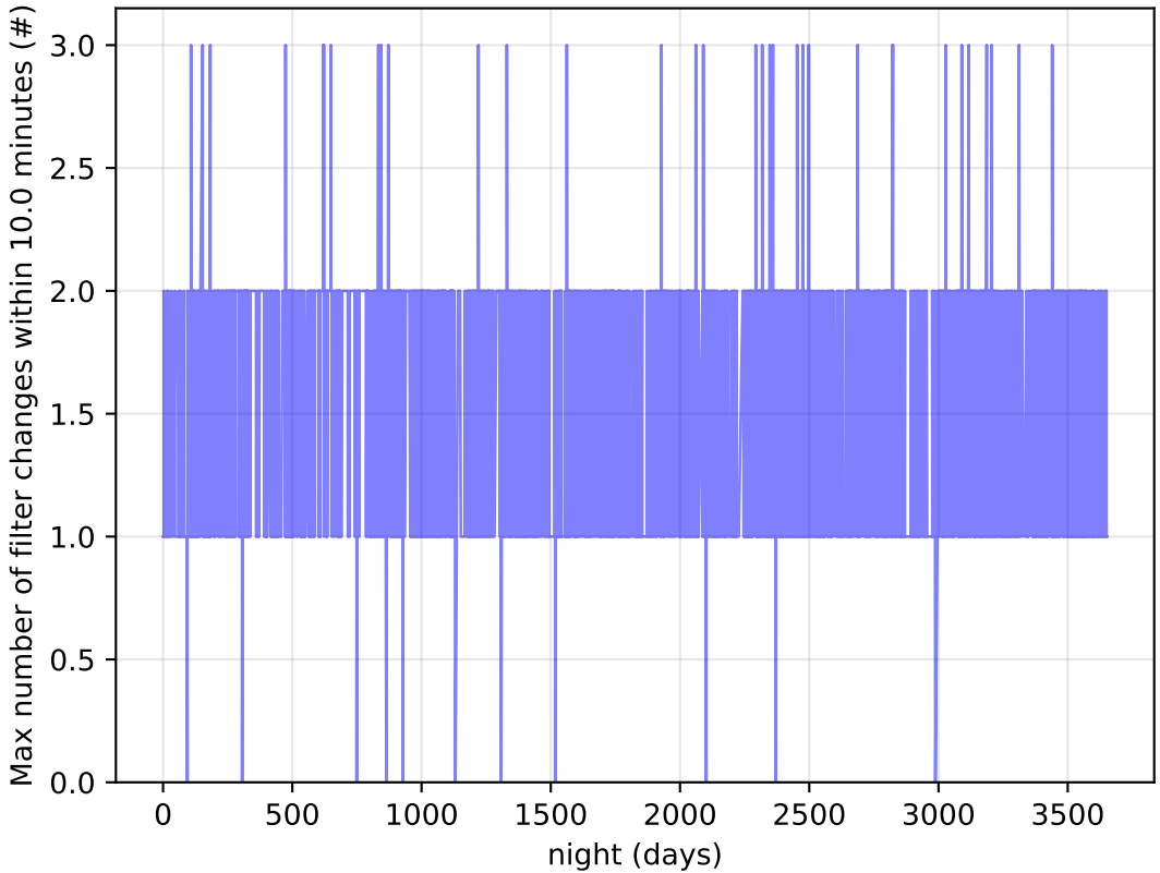
extra_ss_neo4_v3.4_10yrs Per Night: Max number of filter changes within 10.0 minutes
