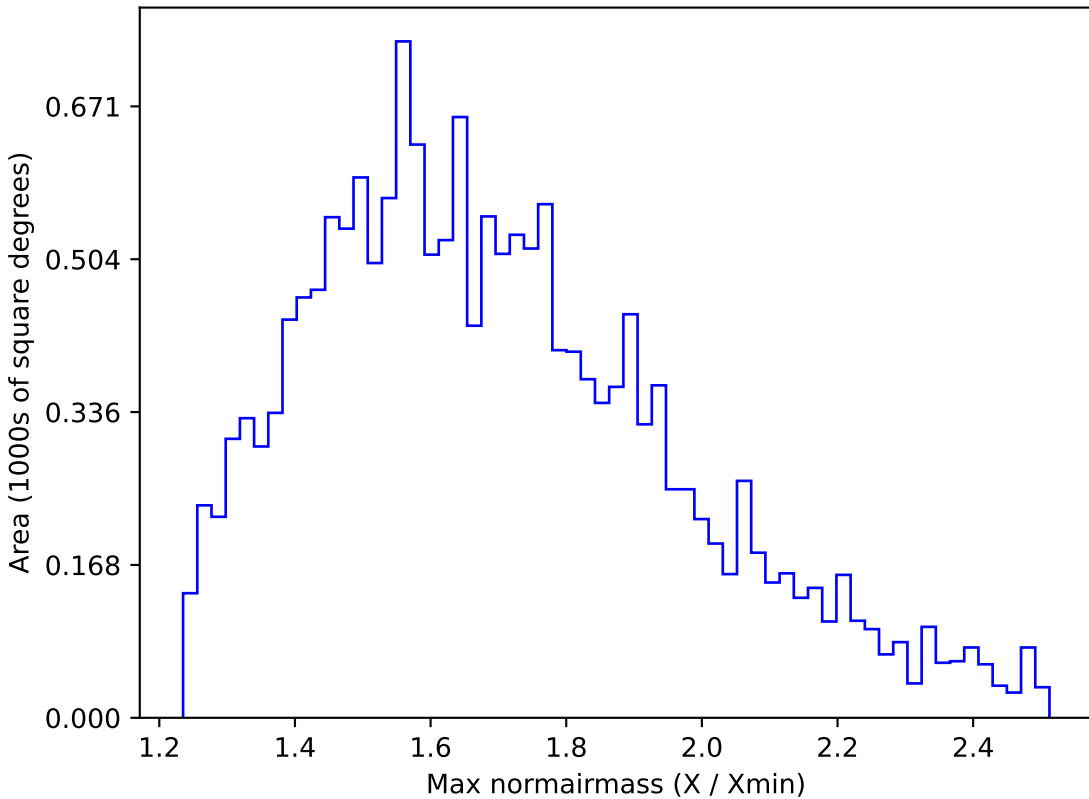
extra_ss_neo4_v3.4_10yrs WFD u band: Max normairmass
