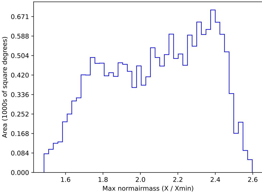
extra_ss_neo4_v3.4_10yrs WFD r band: Max normairmass
