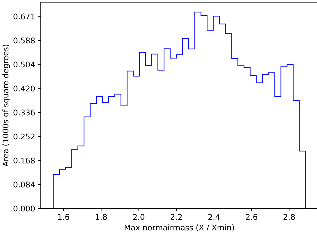
extra_ss_neo4_v3.4_10yrs WFD i band: Max normairmass
