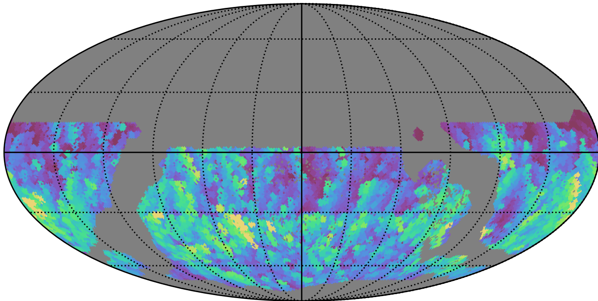
extra_ss_neo4_v3.4_10yrs WFD g band: Max normairmass
