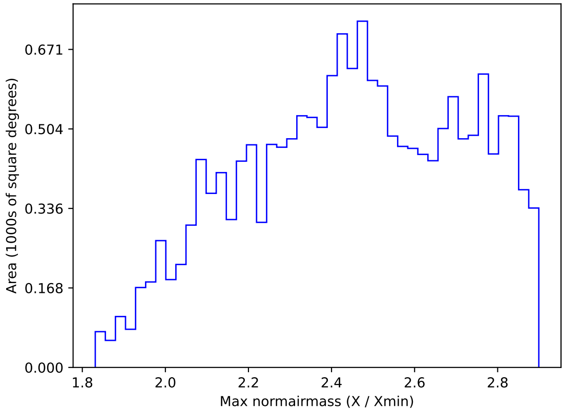
extra_ss_neo4_v3.4_10yrs WFD all bands: Max normairmass
