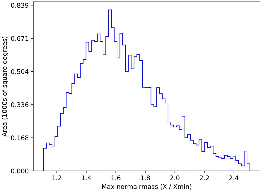
extra_ss_neo4_v3.4_10yrs All sky u band: Max normairmass
