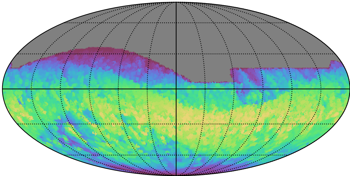
extra_ss_neo4_v3.4_10yrs All sky all bands: Max normairmass
