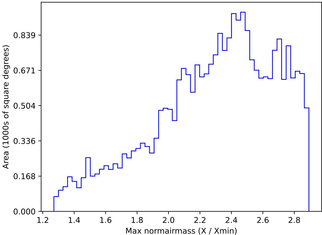
extra_ss_neo4_v3.4_10yrs All sky all bands: Max normairmass
