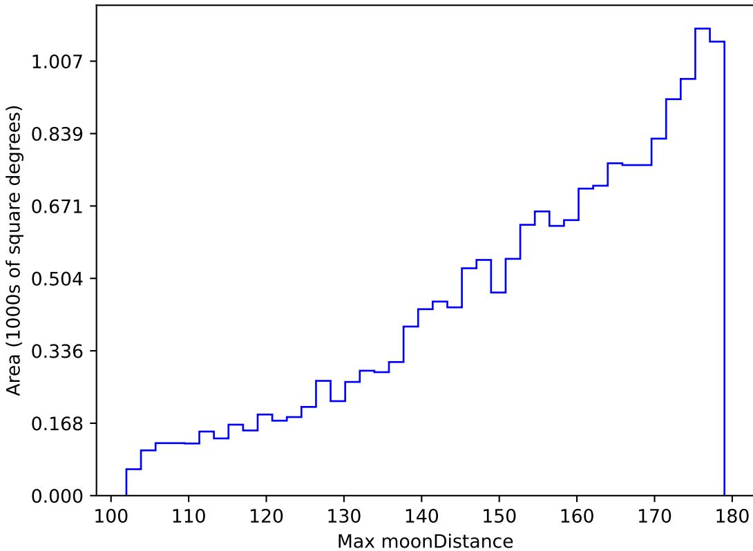
extra_ss_neo4_v3.4_10yrs WFD u band: Max moonDistance
