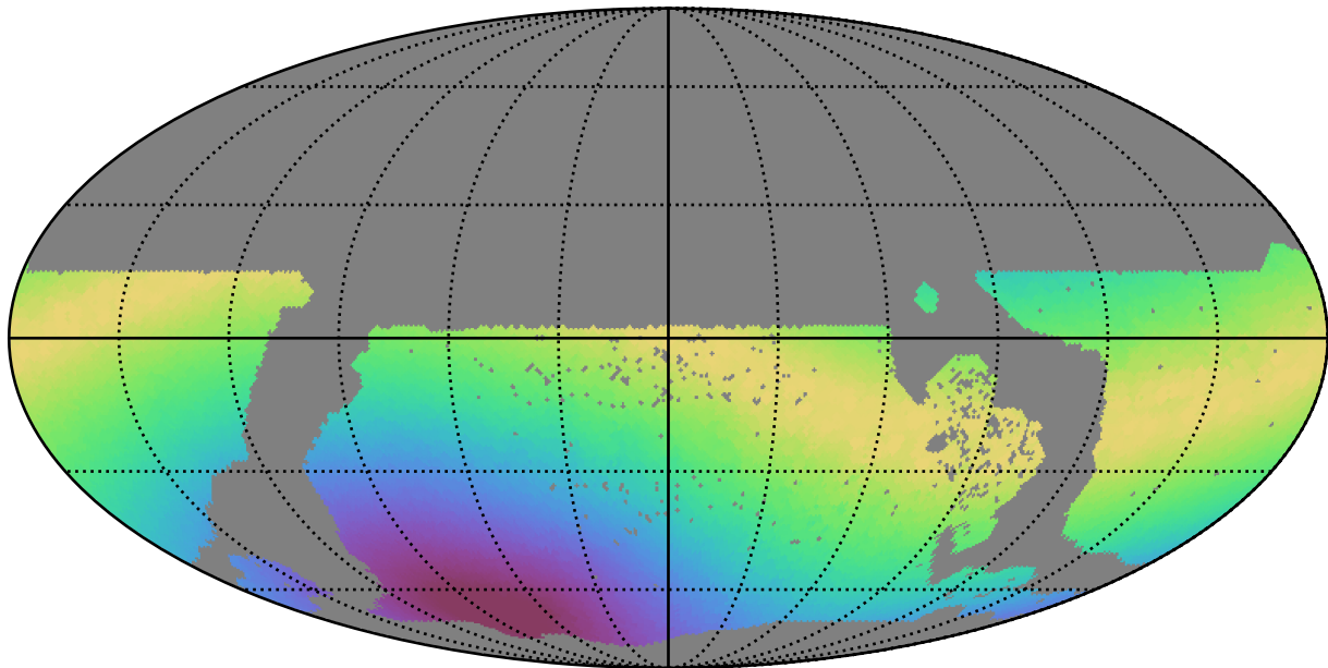
extra_ss_neo4_v3.4_10yrs WFD all bands: Max moonDistance
