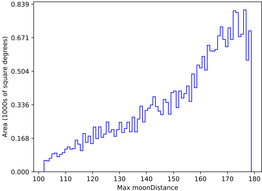
extra_ss_neo4_v3.4_10yrs All sky z band: Max moonDistance
