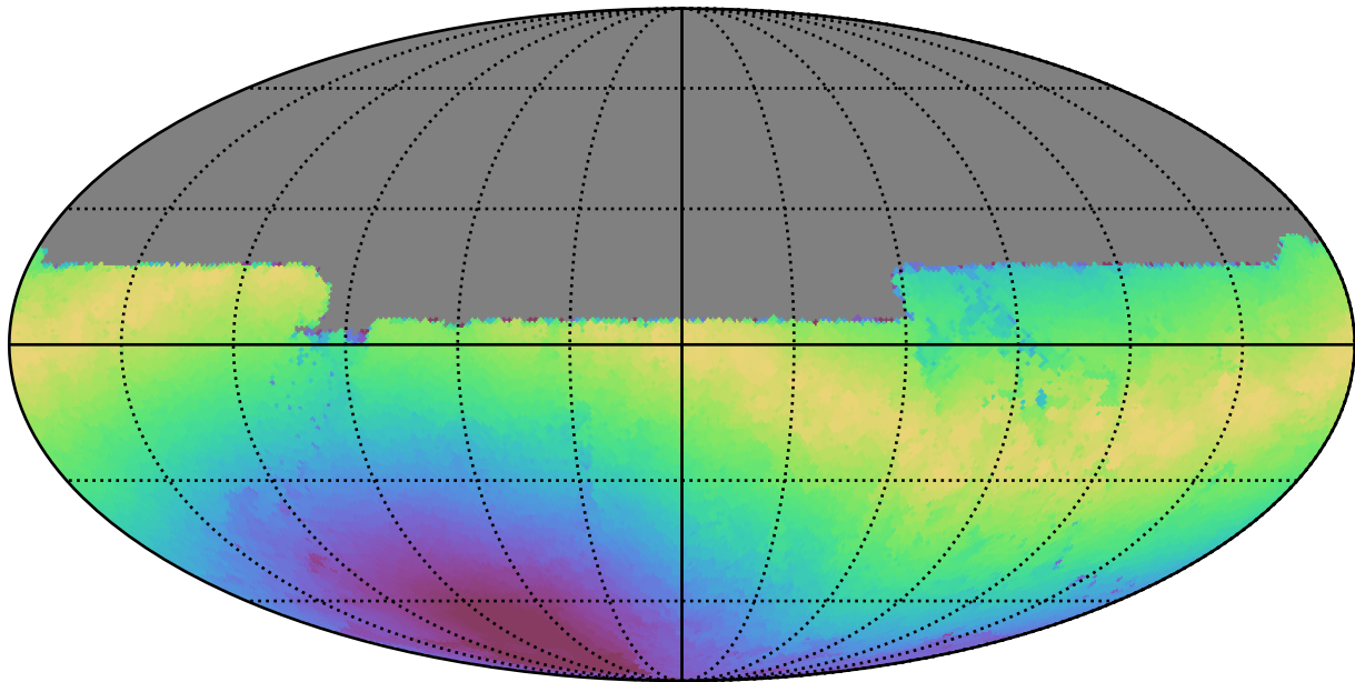
extra_ss_neo4_v3.4_10yrs All sky u band: Max moonDistance
