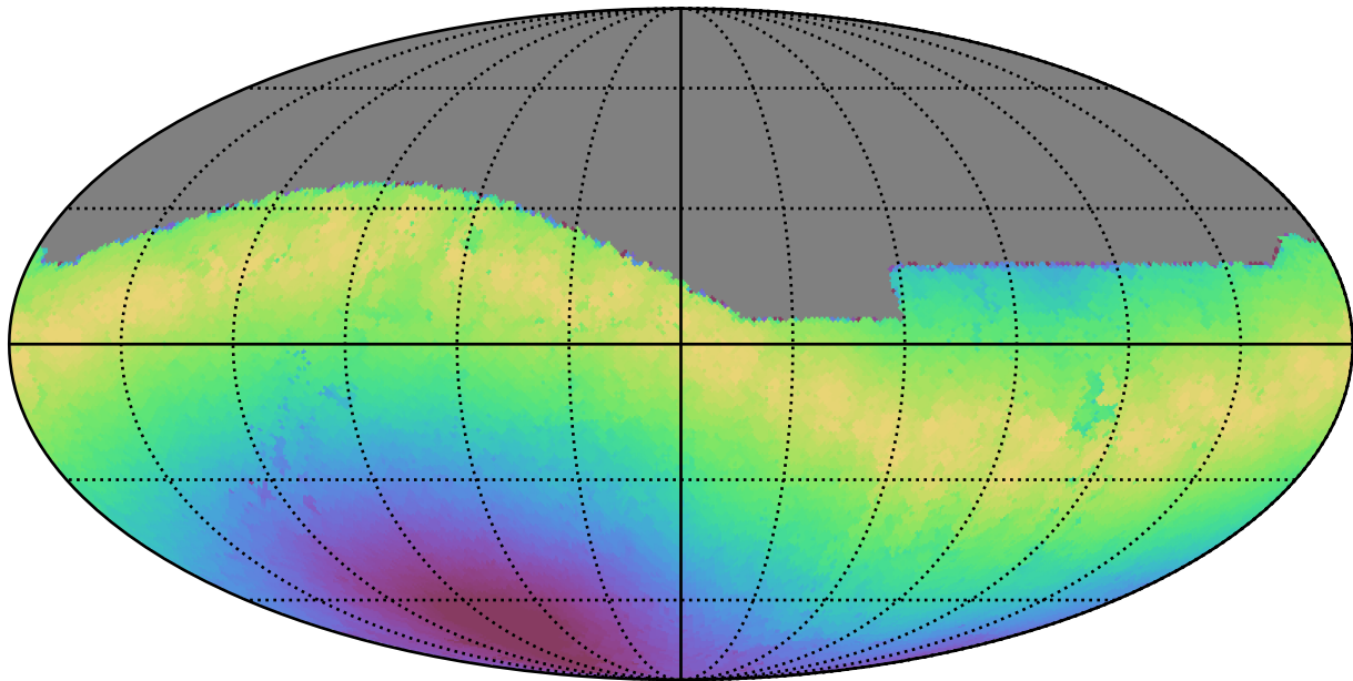
extra_ss_neo4_v3.4_10yrs All sky g band: Max moonDistance
