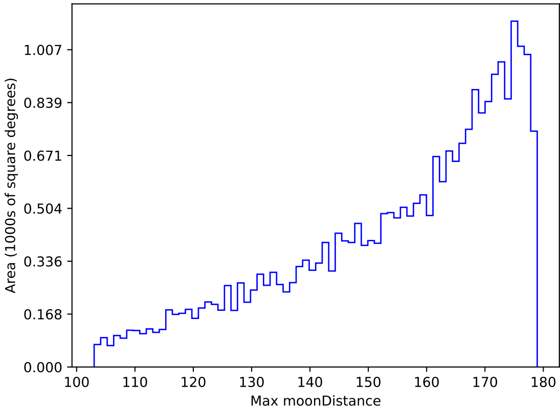
extra_ss_neo4_v3.4_10yrs All sky g band: Max moonDistance
