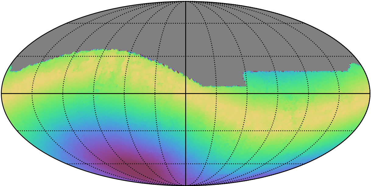
extra_ss_neo4_v3.4_10yrs All sky all bands: Max moonDistance
