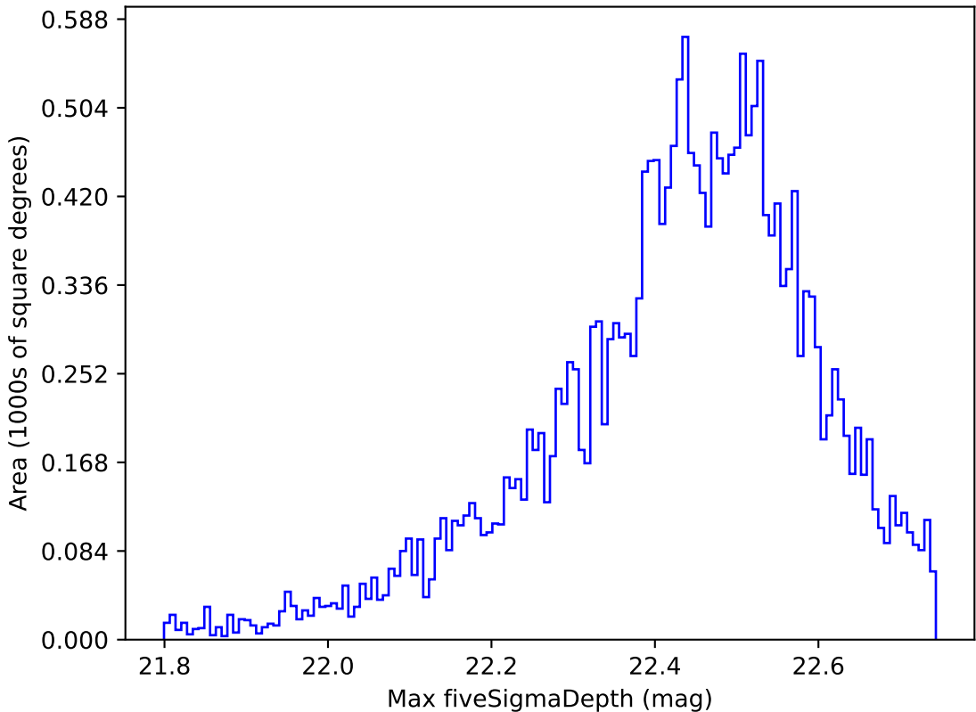
extra_ss_neo4_v3.4_10yrs Yr 1 y band: Max fiveSigmaDepth
