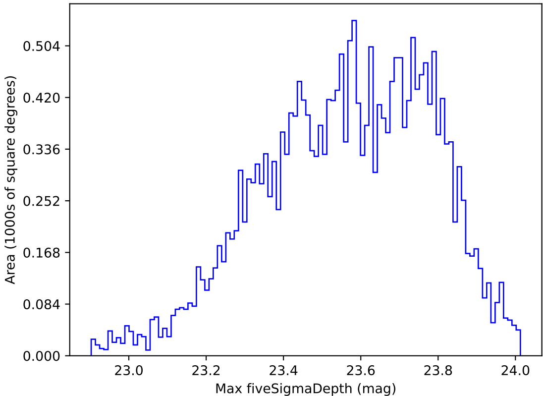
extra_ss_neo4_v3.4_10yrs Yr 1 u band: Max fiveSigmaDepth
