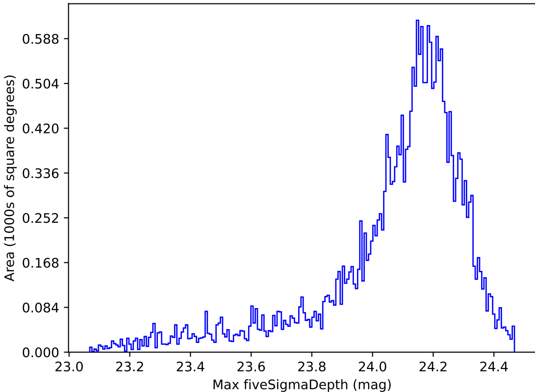
extra_ss_neo4_v3.4_10yrs Yr 1 i band: Max fiveSigmaDepth
