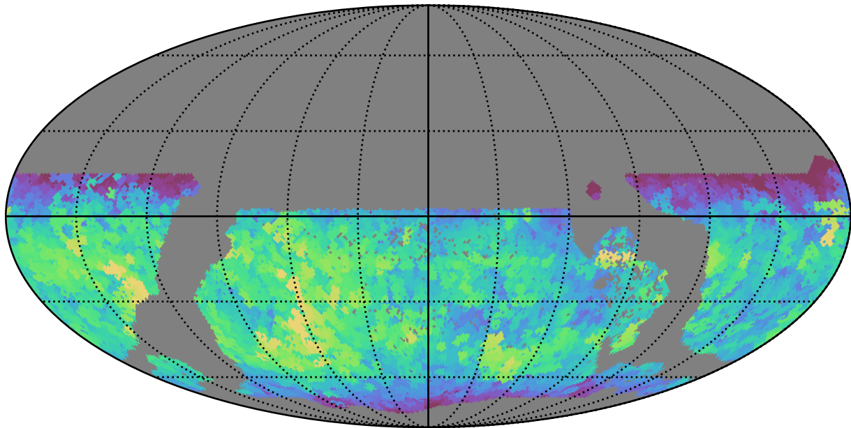
extra_ss_neo4_v3.4_10yrs WFD z band: Max fiveSigmaDepth
