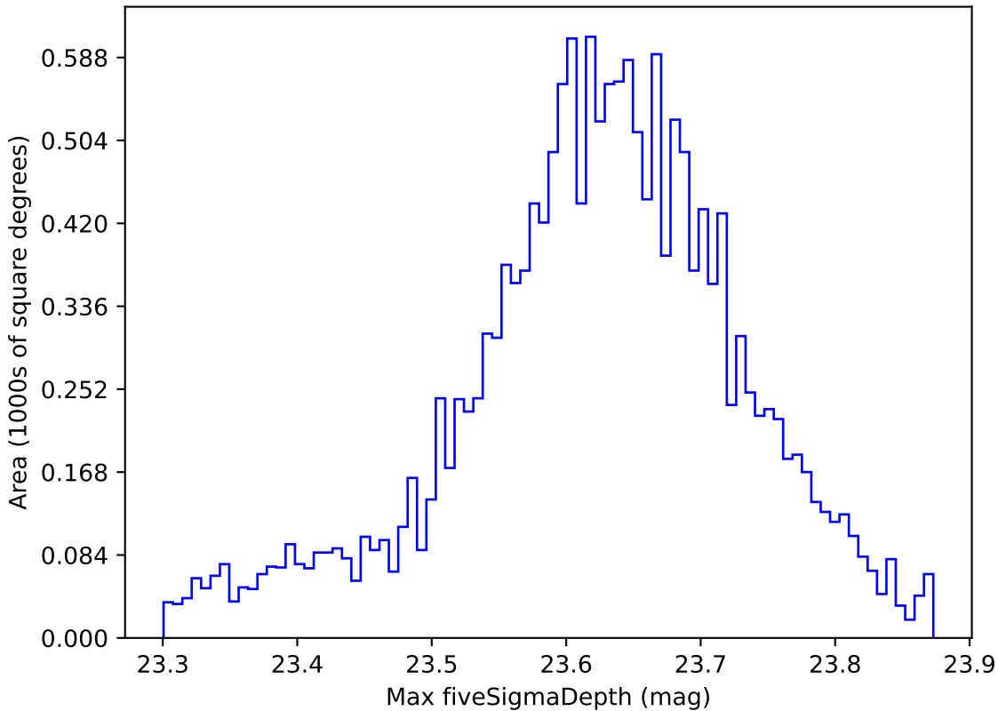
extra_ss_neo4_v3.4_10yrs WFD z band: Max fiveSigmaDepth
