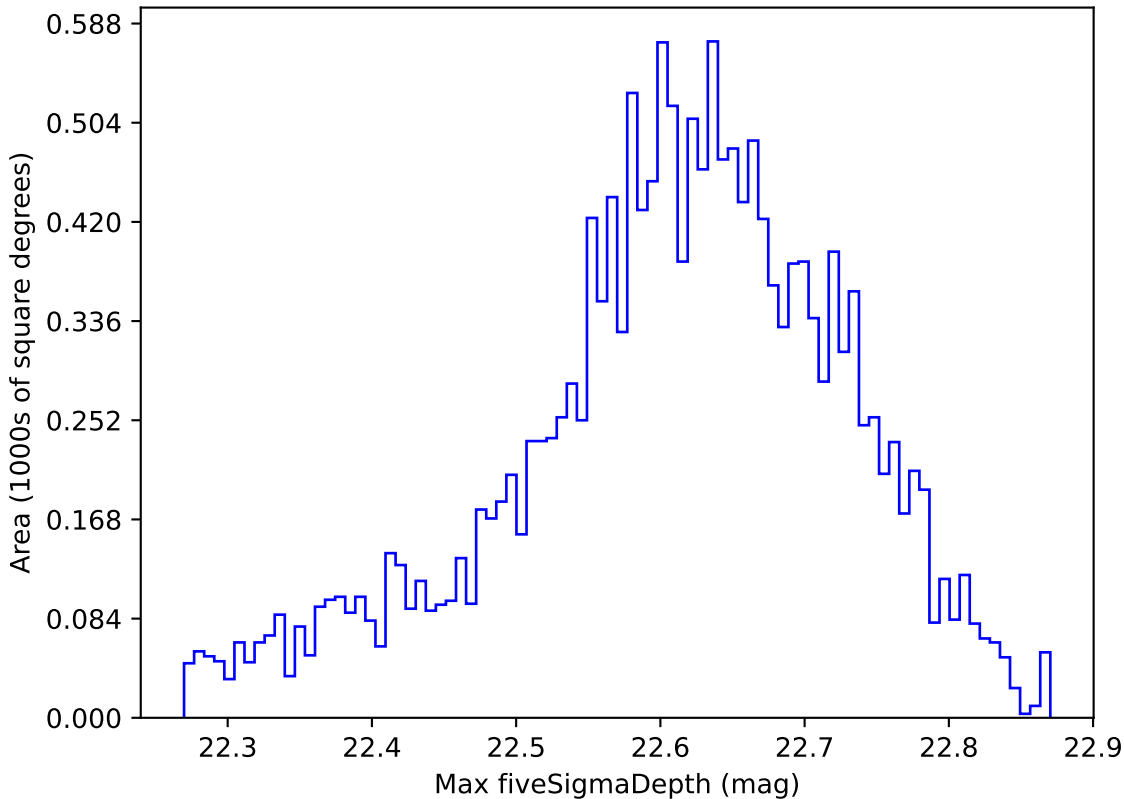
extra_ss_neo4_v3.4_10yrs WFD y band: Max fiveSigmaDepth
