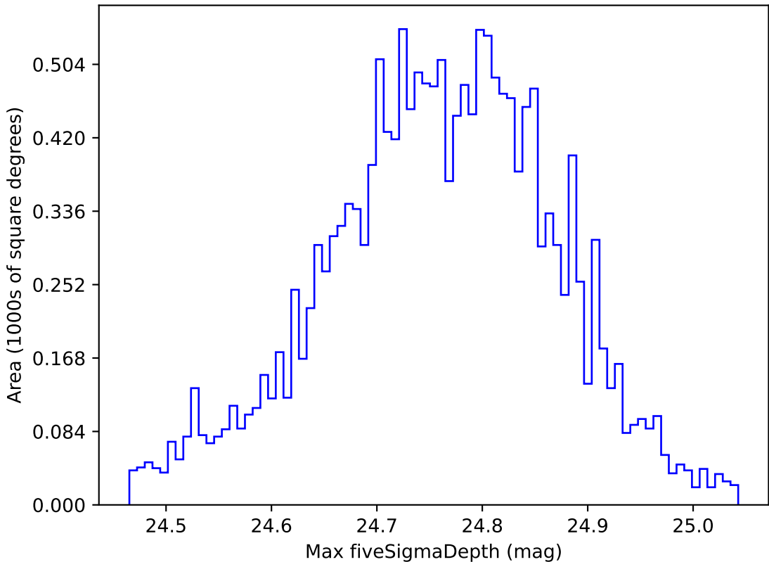
extra_ss_neo4_v3.4_10yrs WFD r band: Max fiveSigmaDepth
