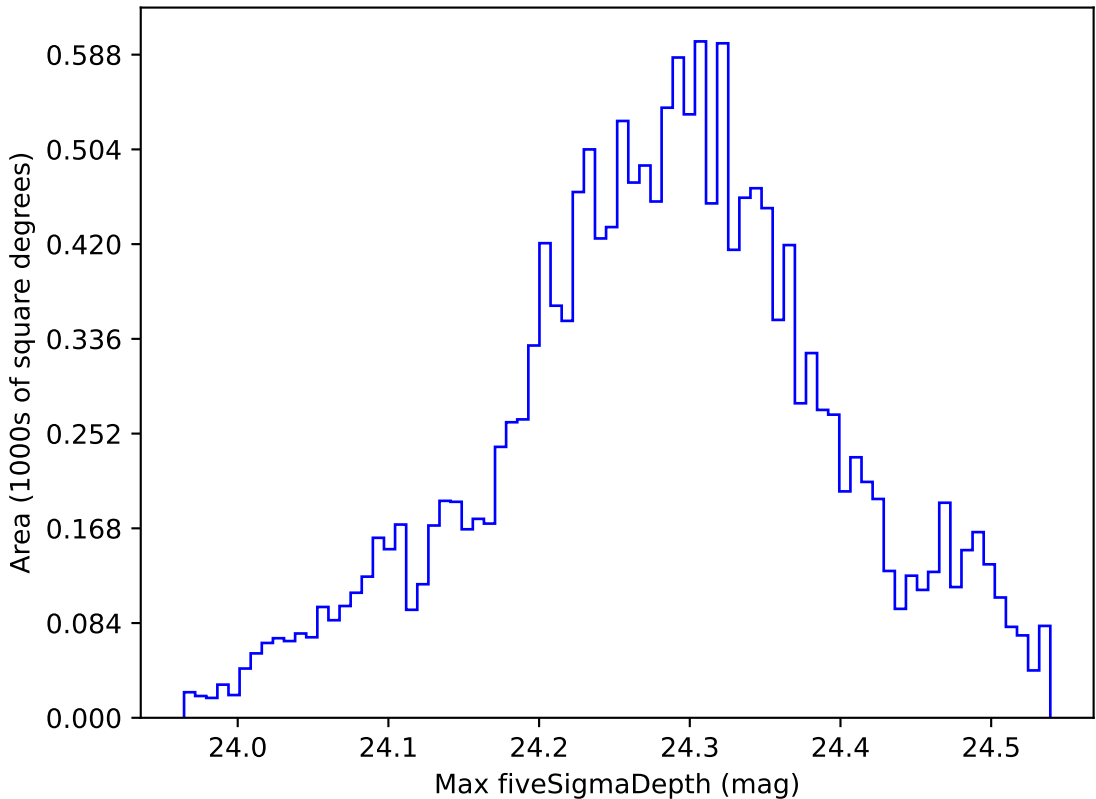
extra_ss_neo4_v3.4_10yrs WFD i band: Max fiveSigmaDepth
