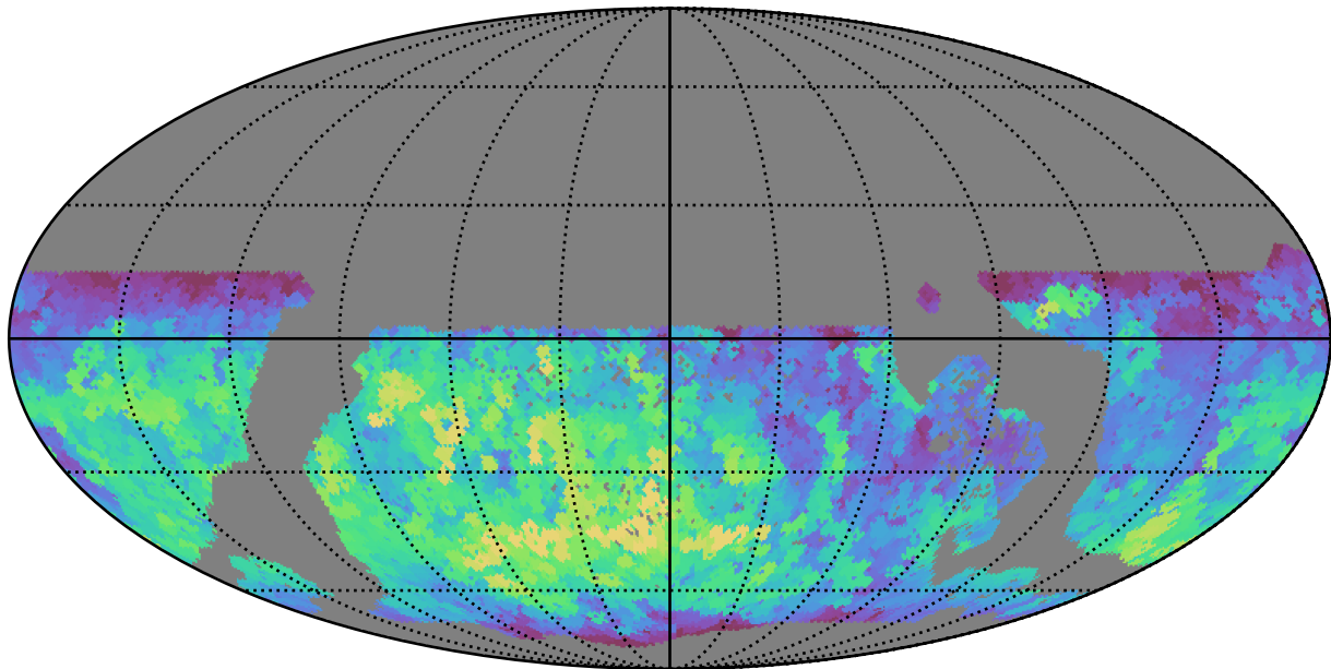
extra_ss_neo4_v3.4_10yrs WFD g band: Max fiveSigmaDepth
