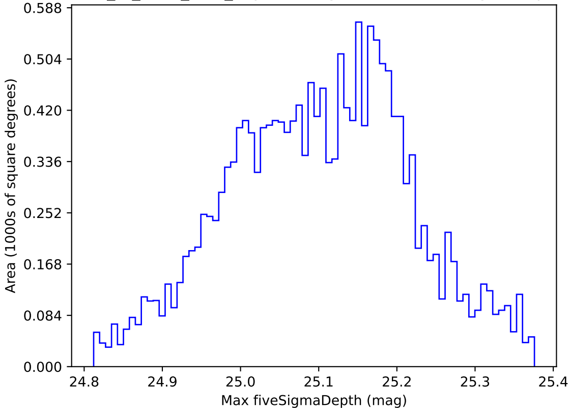
extra_ss_neo4_v3.4_10yrs WFD g band: Max fiveSigmaDepth
