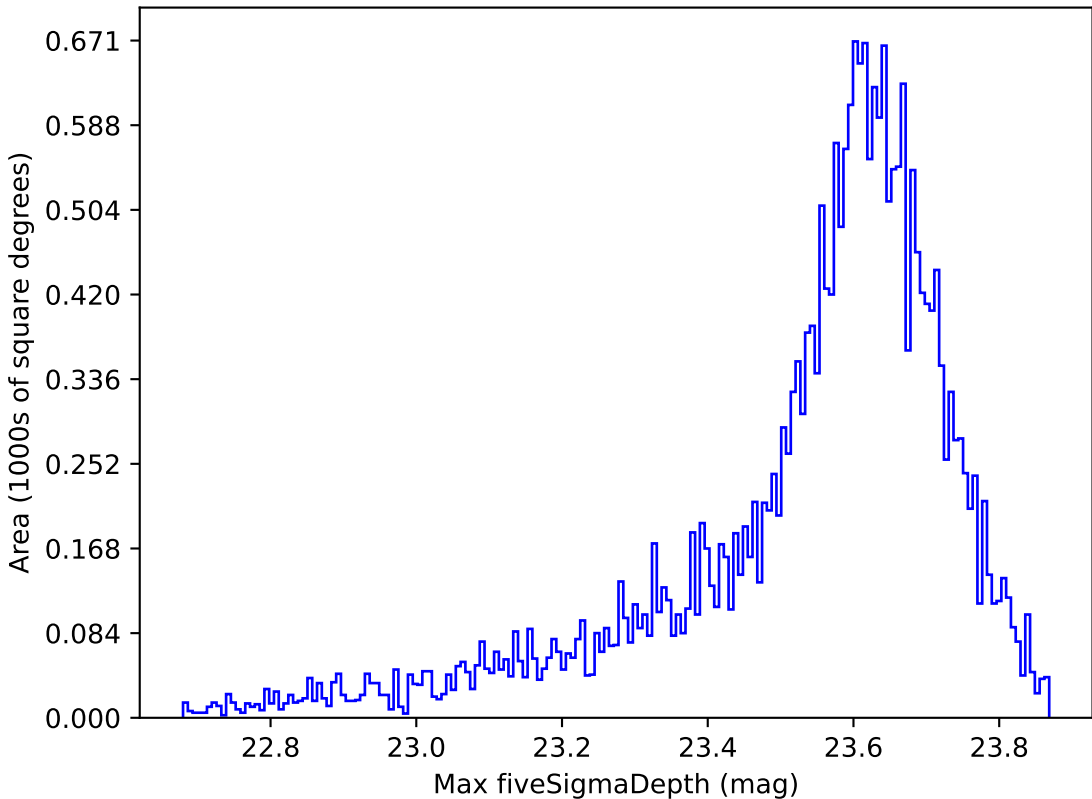
extra_ss_neo4_v3.4_10yrs All sky z band: Max fiveSigmaDepth
