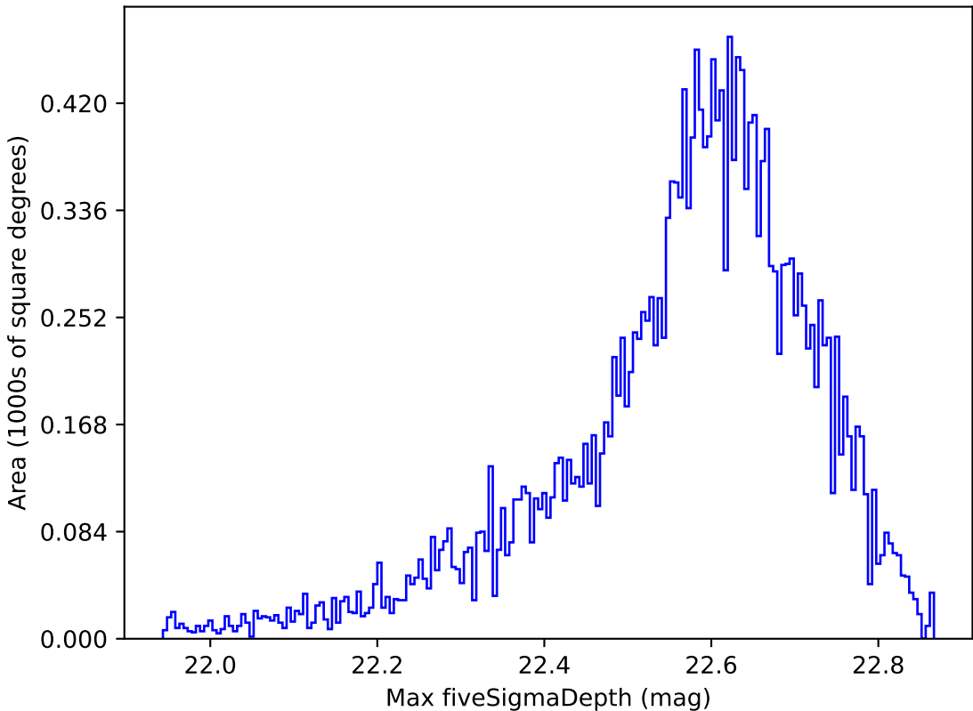
extra_ss_neo4_v3.4_10yrs All sky y band: Max fiveSigmaDepth
