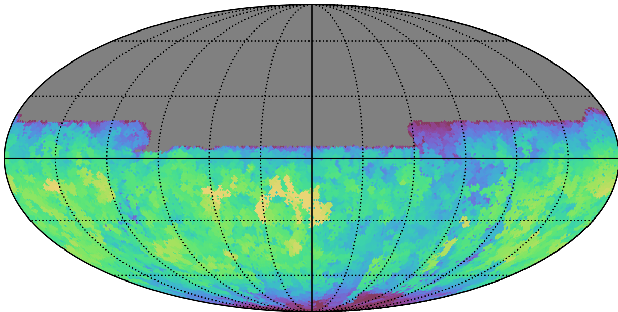
extra_ss_neo4_v3.4_10yrs All sky u band: Max fiveSigmaDepth
