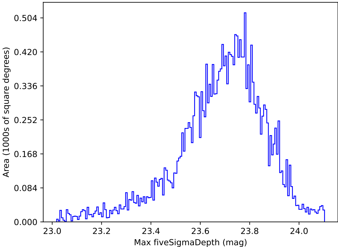
extra_ss_neo4_v3.4_10yrs All sky u band: Max fiveSigmaDepth
