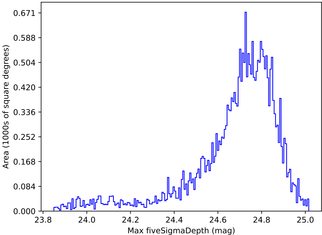
extra_ss_neo4_v3.4_10yrs All sky r band: Max fiveSigmaDepth
