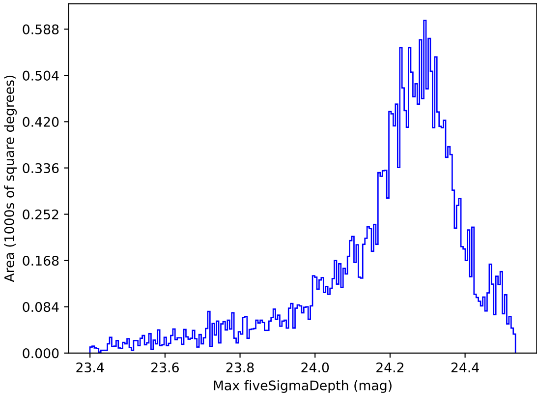
extra_ss_neo4_v3.4_10yrs All sky i band: Max fiveSigmaDepth
