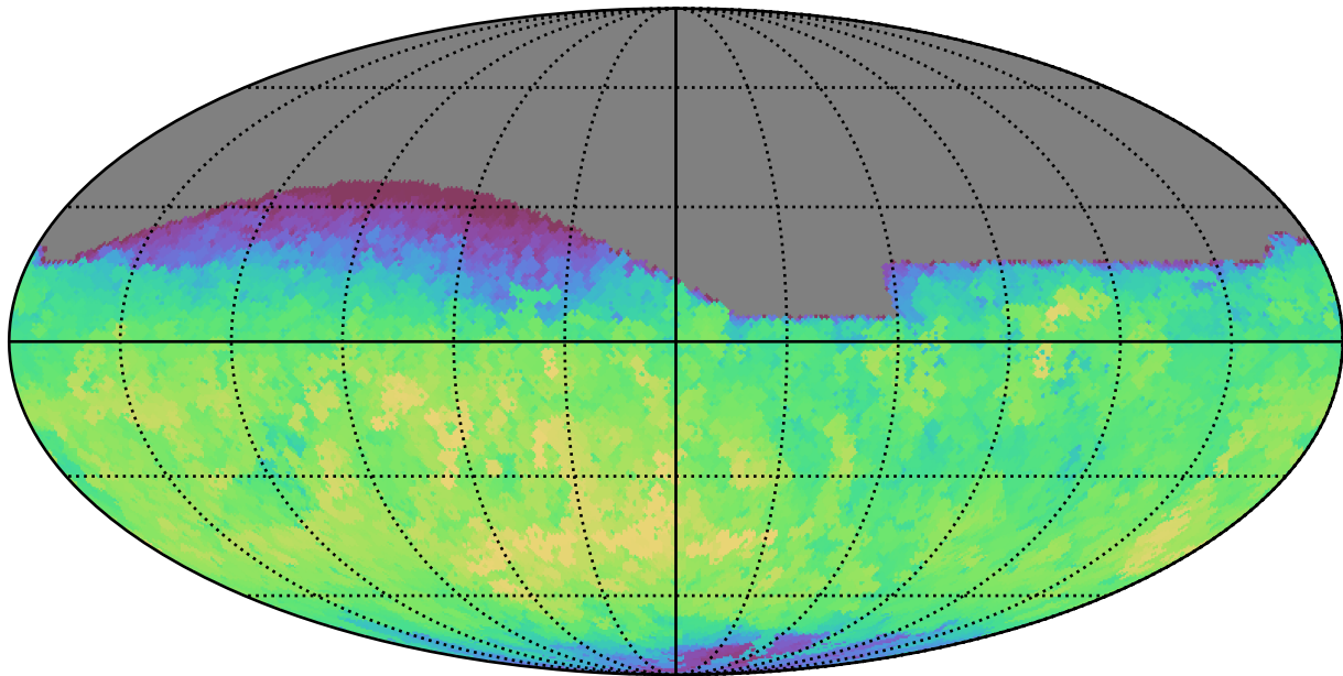
extra_ss_neo4_v3.4_10yrs All sky g band: Max fiveSigmaDepth
