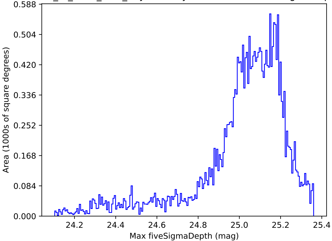
extra_ss_neo4_v3.4_10yrs All sky all bands: Max fiveSigmaDepth
