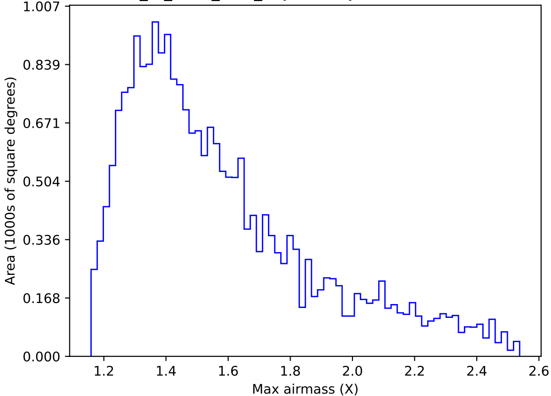
extra_ss_neo4_v3.4_10yrs Yr 1 y band: Max airmass
