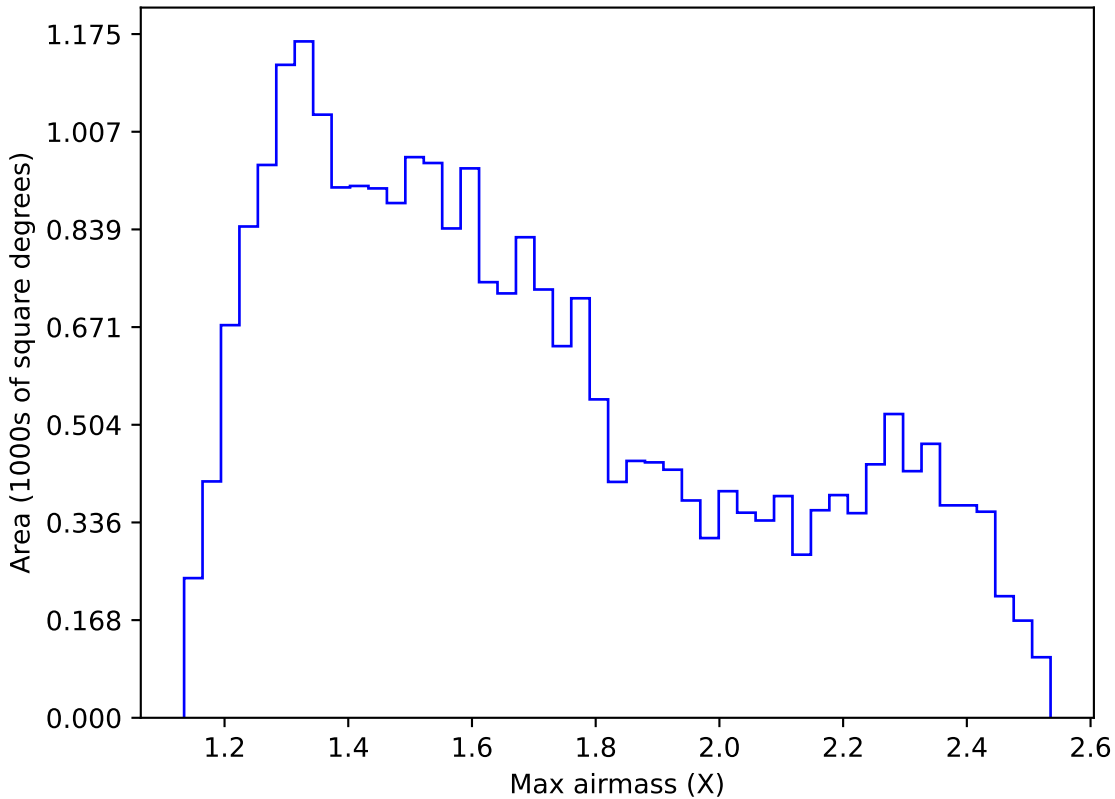
extra_ss_neo4_v3.4_10yrs Yr 1 r band: Max airmass
