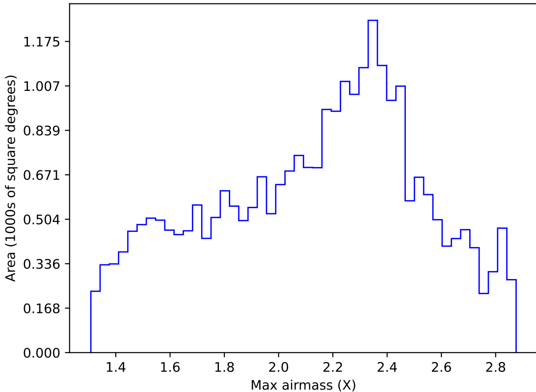
extra_ss_neo4_v3.4_10yrs Yr 1 all bands: Max airmass
