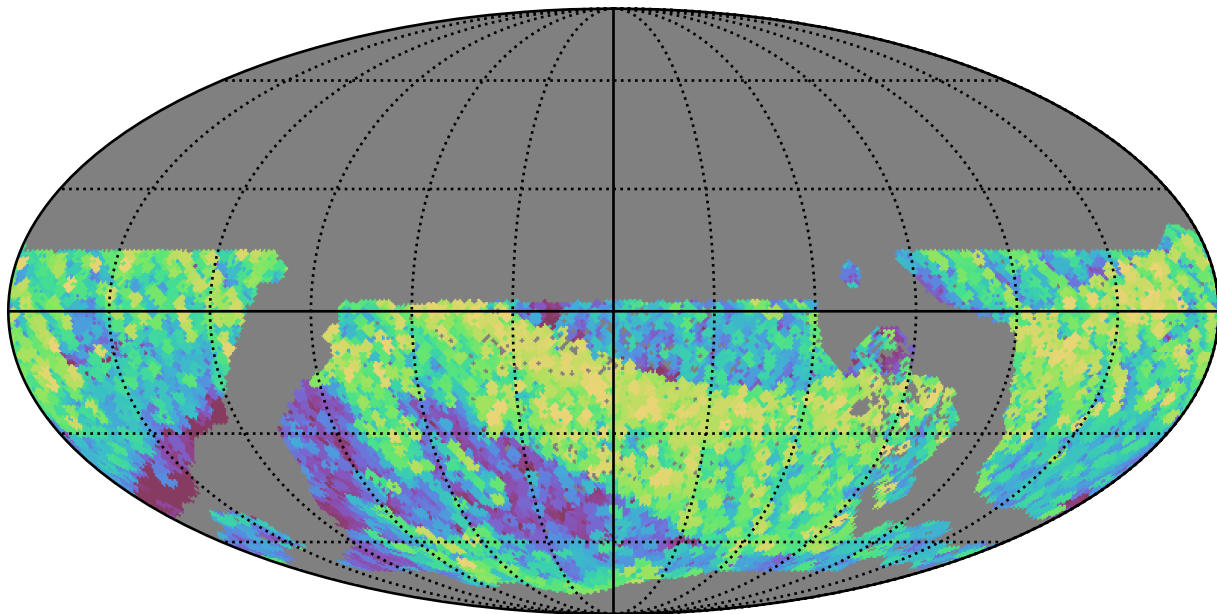
extra_ss_neo4_v3.4_10yrs WFD z band: Max airmass
