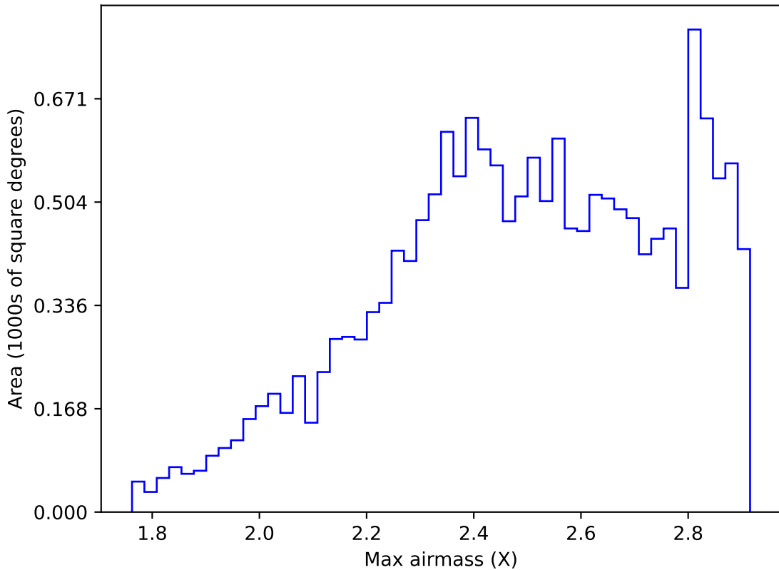
extra_ss_neo4_v3.4_10yrs WFD z band: Max airmass
