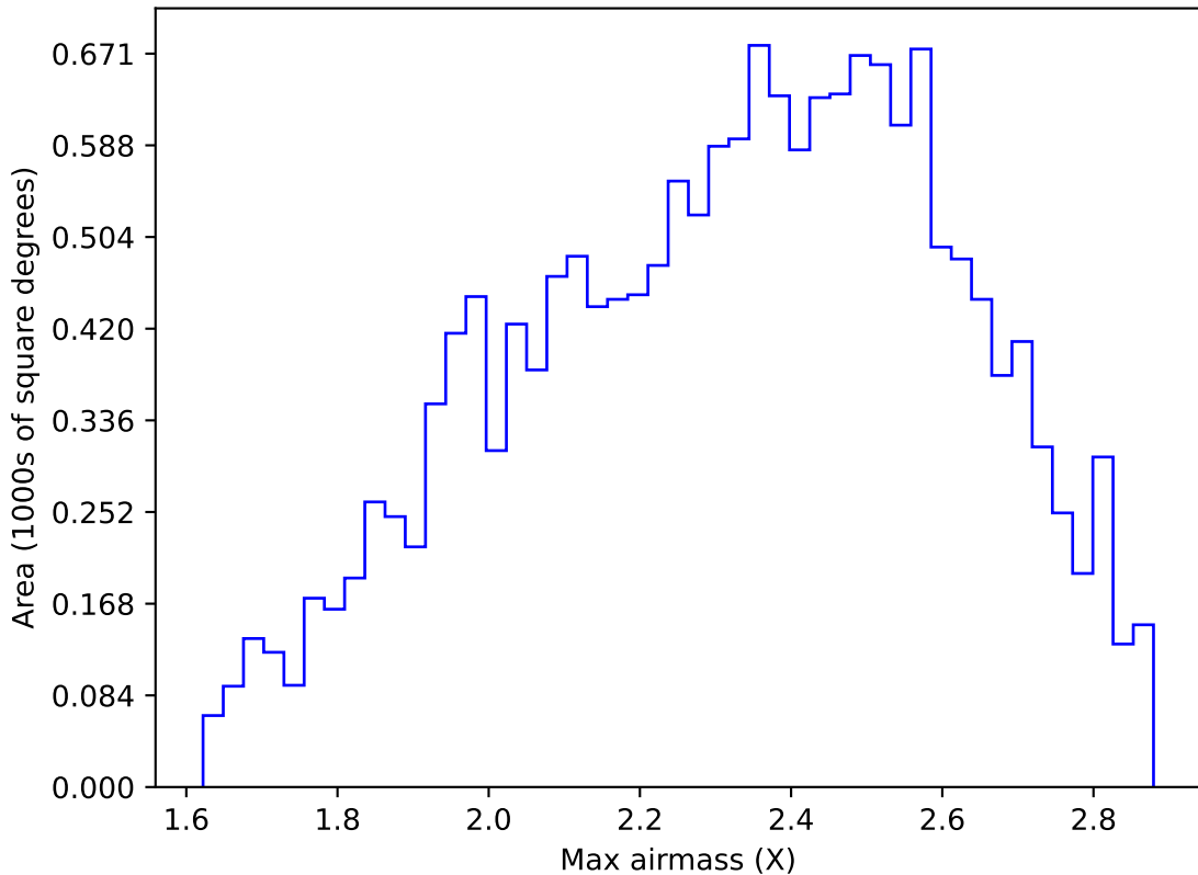
extra_ss_neo4_v3.4_10yrs WFD y band: Max airmass
